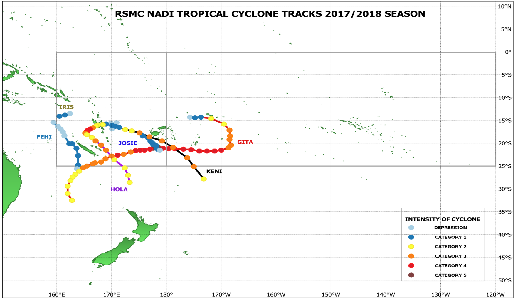
Figure 10: Analogue season track map – 2017-18 season
